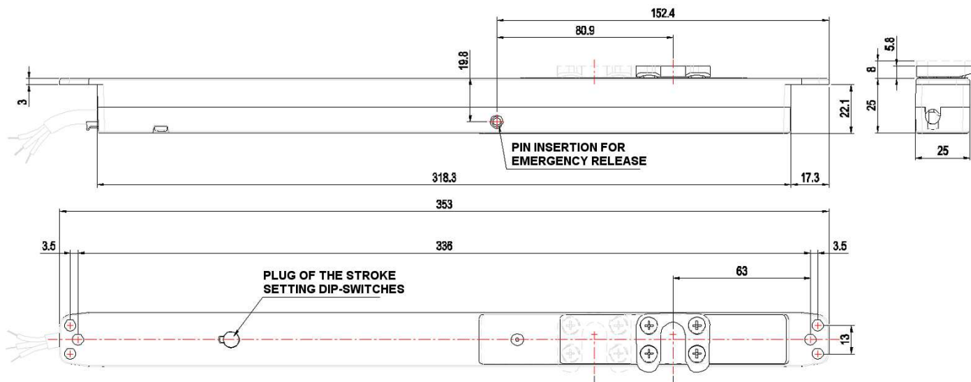
General dimensions of the linear electrical actuator
