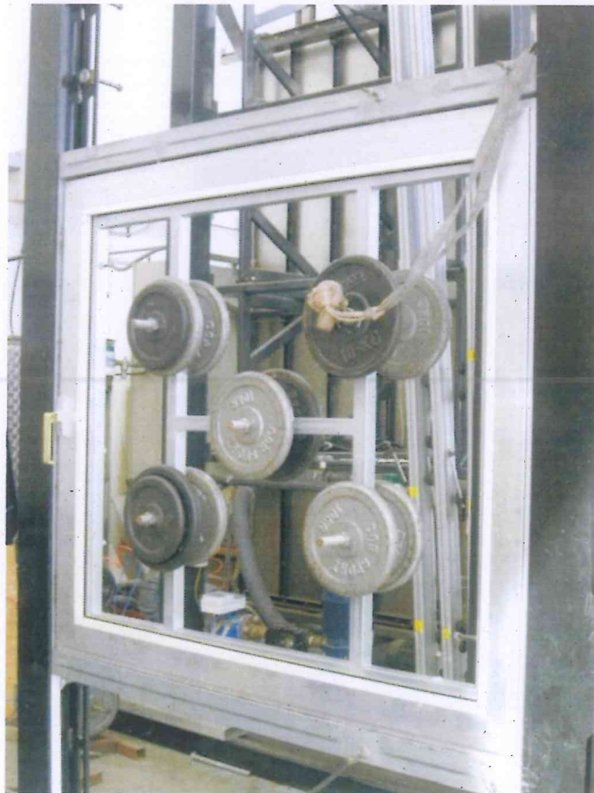
Photo 1. Tested sample in the experimental setup.
