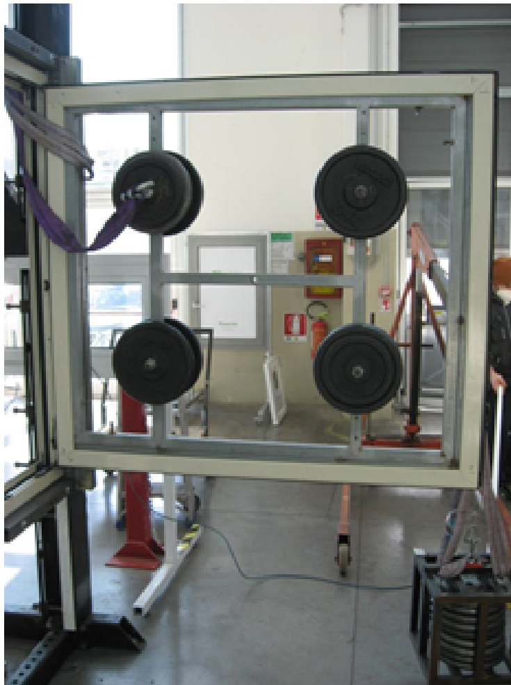
Photo 1 Tested sample during the additional loading
